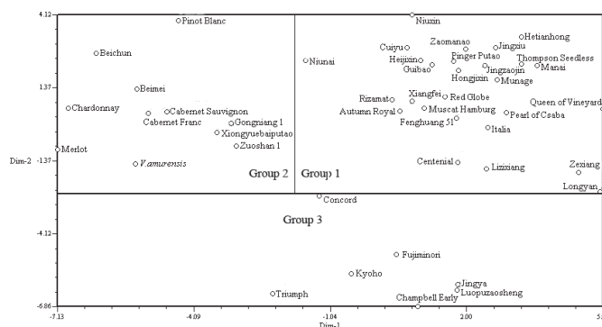
Fig. 2. Two-dimensional projection of the principal component analysis of 45 grape varieties based on 9 SSR markers along the first two principal axes
